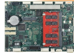
Rugged SBC used in ATR system
