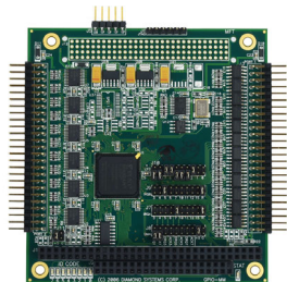
Digital I/O PC/104
