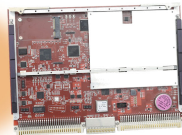
Rugged custom VME64x SBC used on US Army M1 tank
